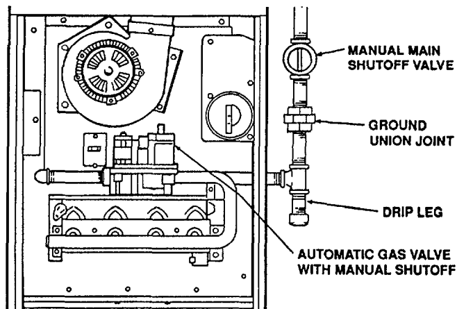
RIGHT SIDE PIPING (OPTIONAL)
