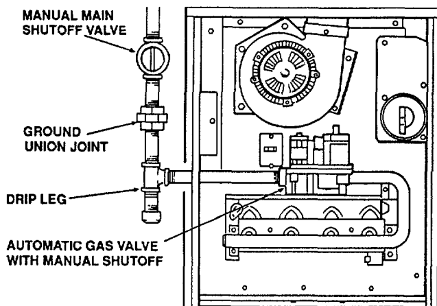
LEFT SIDE PIPING (STANDARD)
